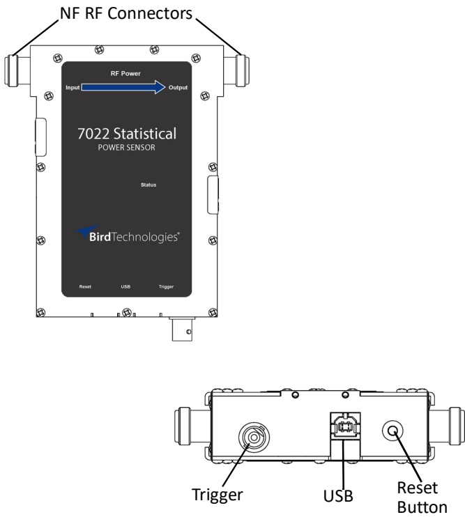
Figure 1 Sensor Outline
